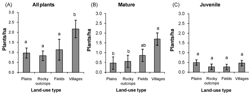
Fig. 3. Density (mean ± SE) of all plants (A), mature (B) and juvenile (C) baobab populations in different land-use types. Bars marked with different letters (a and b) are significantly different (Fisher's LSD, p < 0.05 ).
